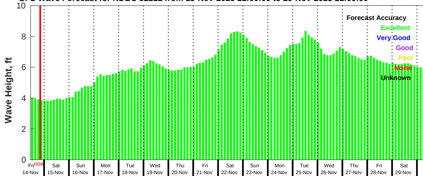
GFS Wave Forecast for NDBC 52211 from 13-Nov-2025 11:00:00 to 29-Nov-2025 11:00:00
