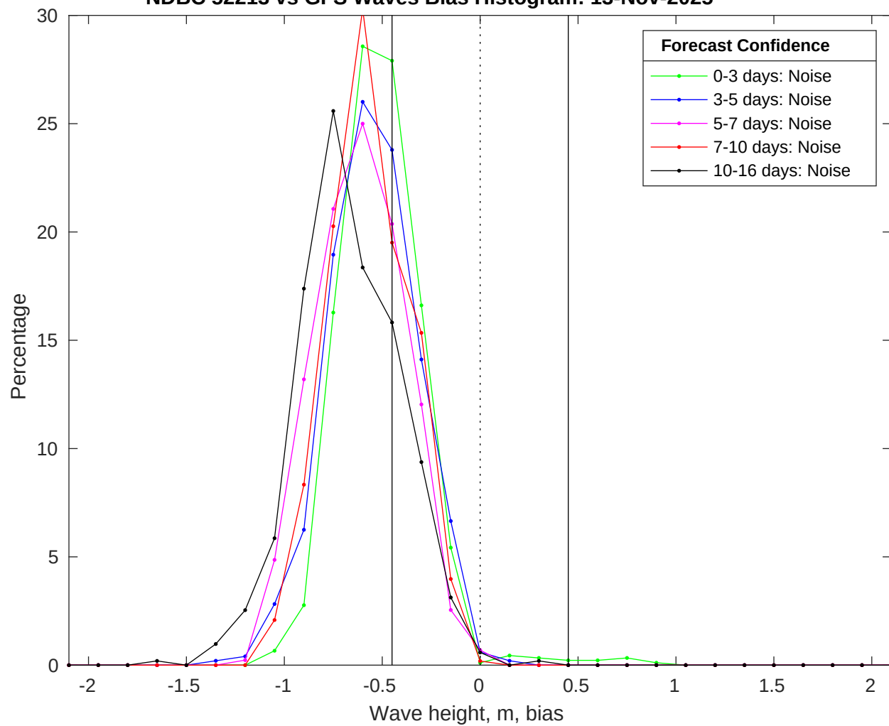
NDBC 52213 vs GFS Waves Bias Histogram: 13-Nov-2025
