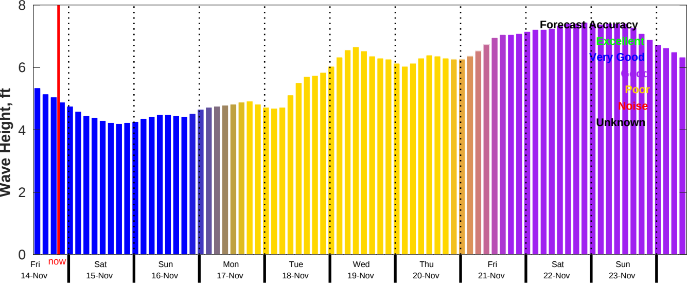
CMEMS Wave Forecast for NDBC 52213 from 13-Nov-2025 11:00:00 to 23-Nov-2025 11:00:00
