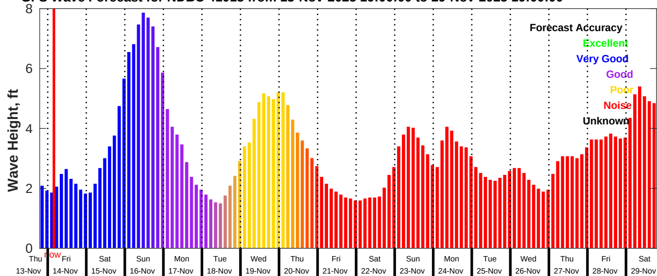
GFS Wave Forecast for NDBC 41013 from 13-Nov-2025 19:00:00 to 29-Nov-2025 19:00:00
