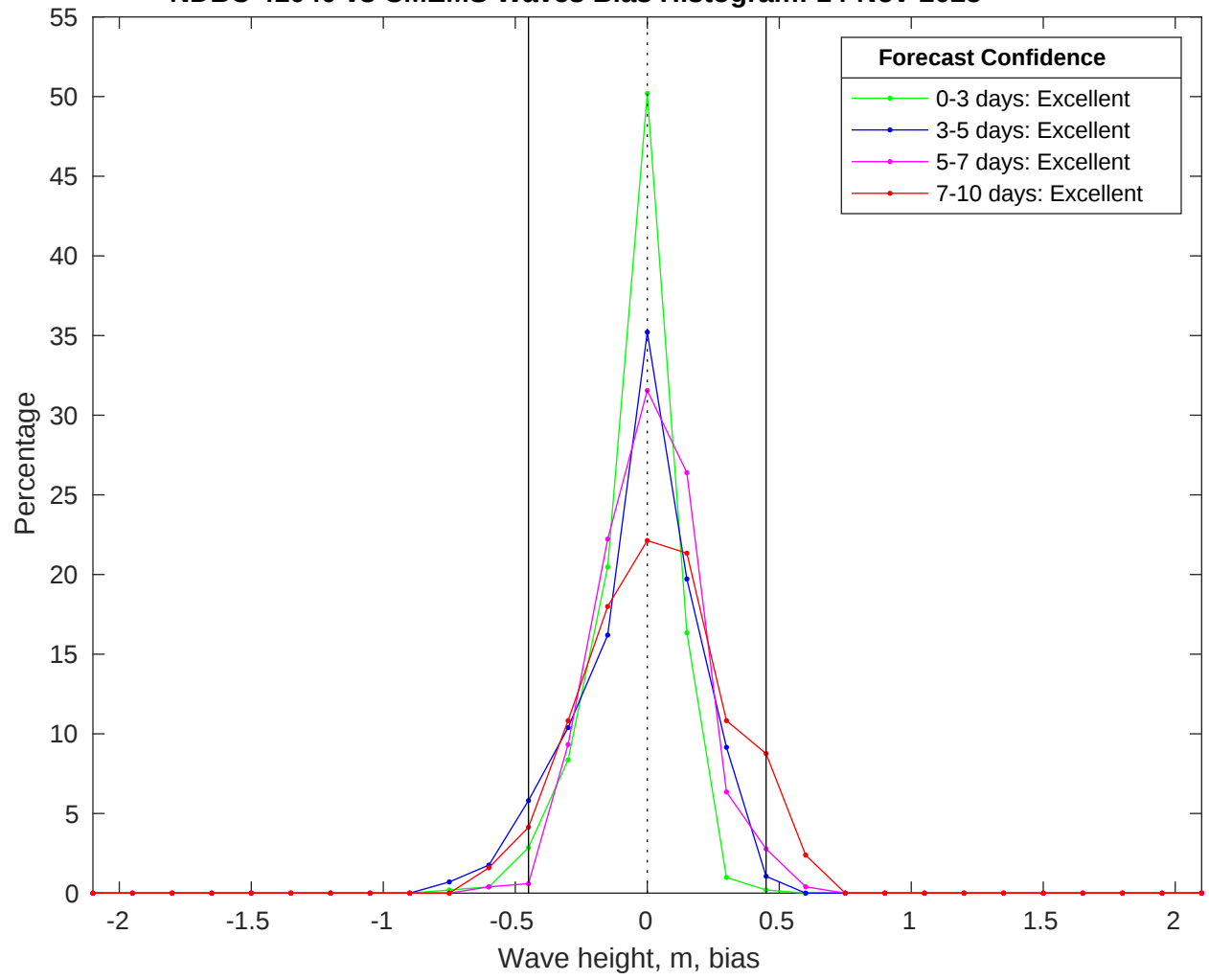
NDBC 41040 vs CMEMS Waves Bias Histogram: 14-Nov-2025
