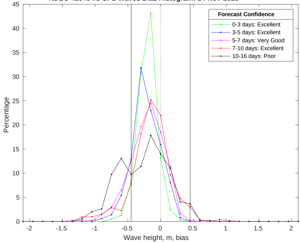
NDBC 41040 vs GFS Waves Bias Histogram: 14-Nov-2025
