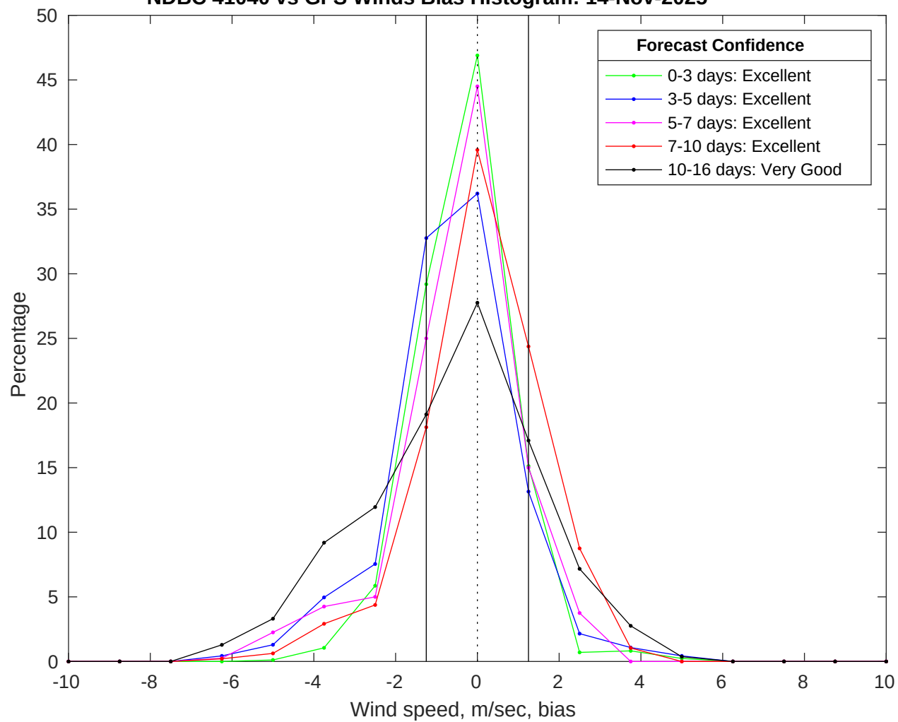
NDBC 41040 vs GFS Winds Bias Histogram: 14-Nov-2025
