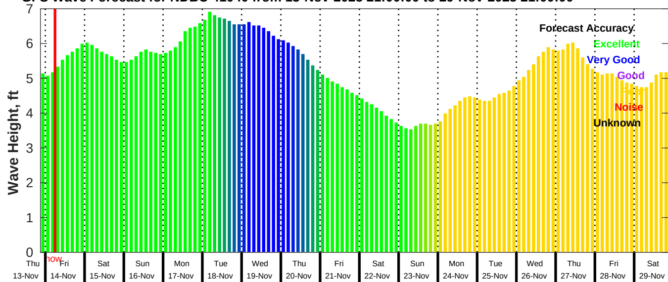
GFS Wave Forecast for NDBC 41040 from 13-Nov-2025 21:00:00 to 29-Nov-2025 21:00:00
