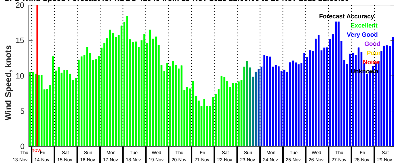
GFS Wind Speed Forecast for NDBC 41040 from 13-Nov-2025 21:00:00 to 29-Nov-2025 21:00:00
