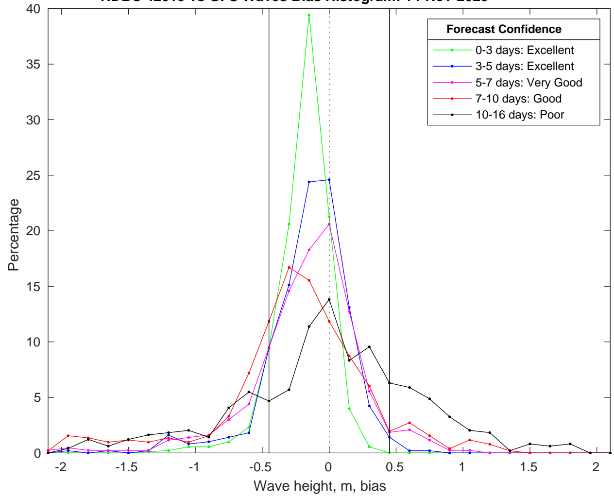
NDBC 42019 vs GFS Waves Bias Histogram: 14-Nov-2025
