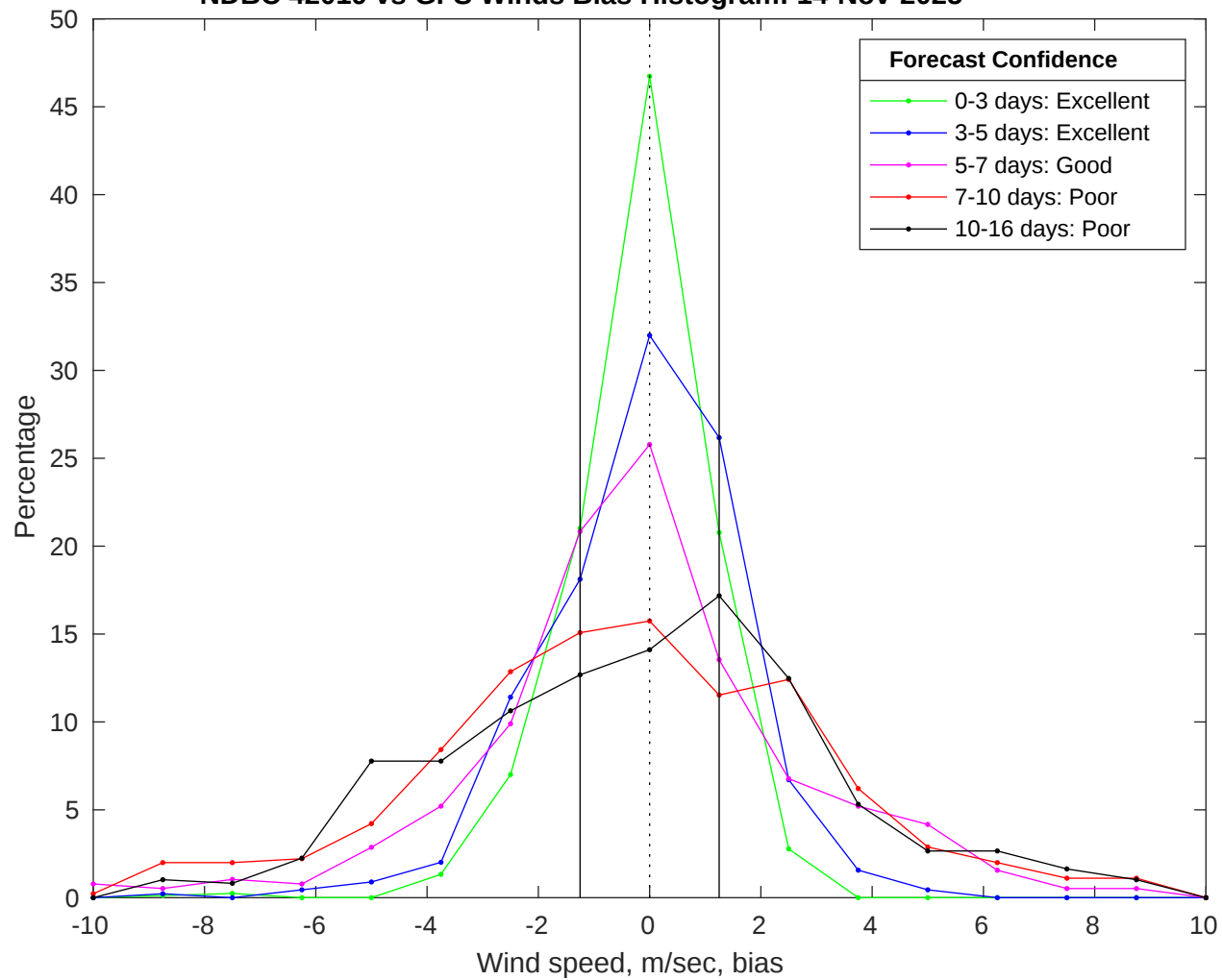
NDBC 42019 vs GFS Winds Bias Histogram: 14-Nov-2025
