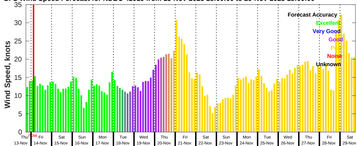
GFS Wind Speed Forecast for NDBC 42019 from 13-Nov-2025 18:00:00 to 29-Nov-2025 18:00:00
