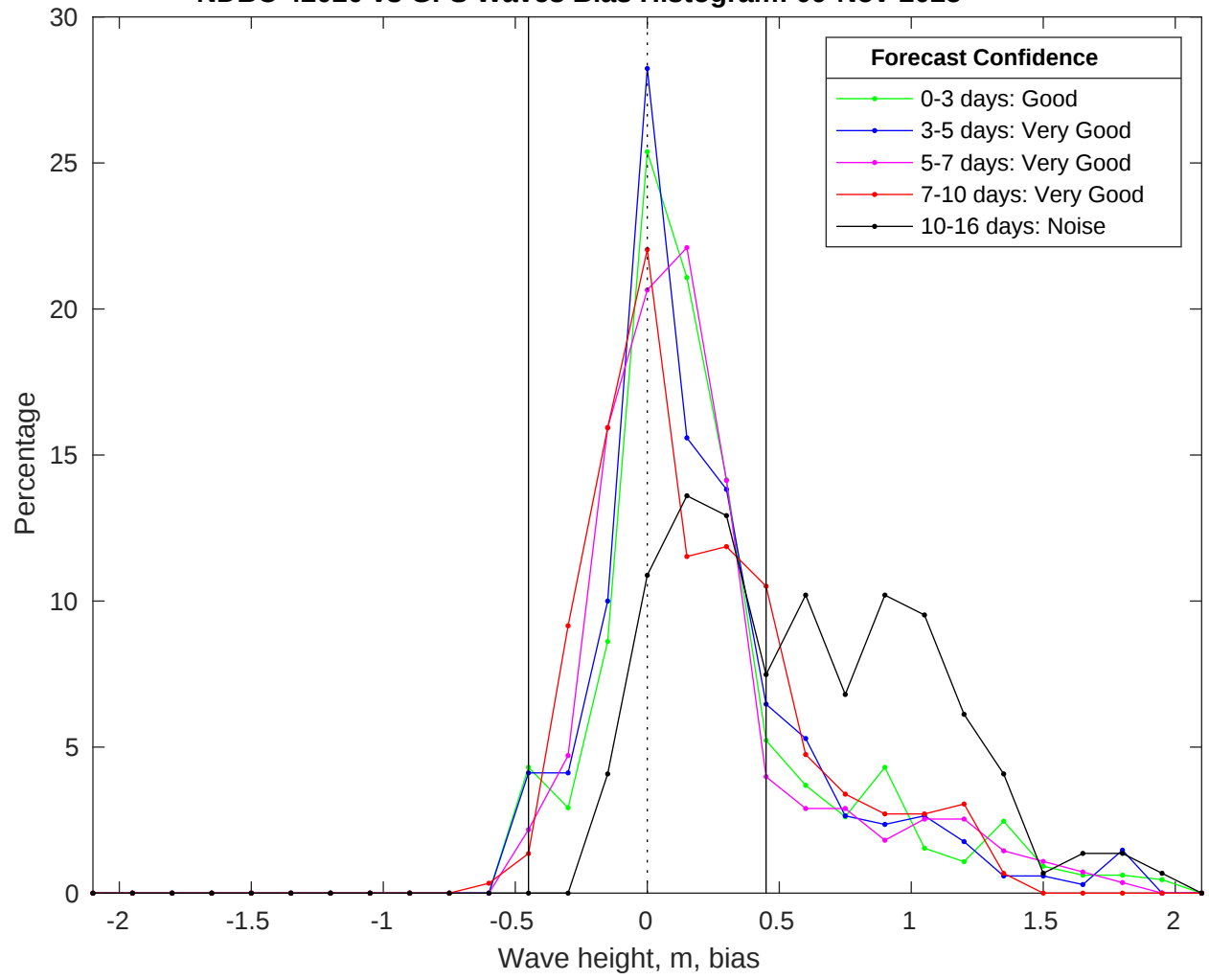
NDBC 42020 vs GFS Waves Bias Histogram: 09-Nov-2025
