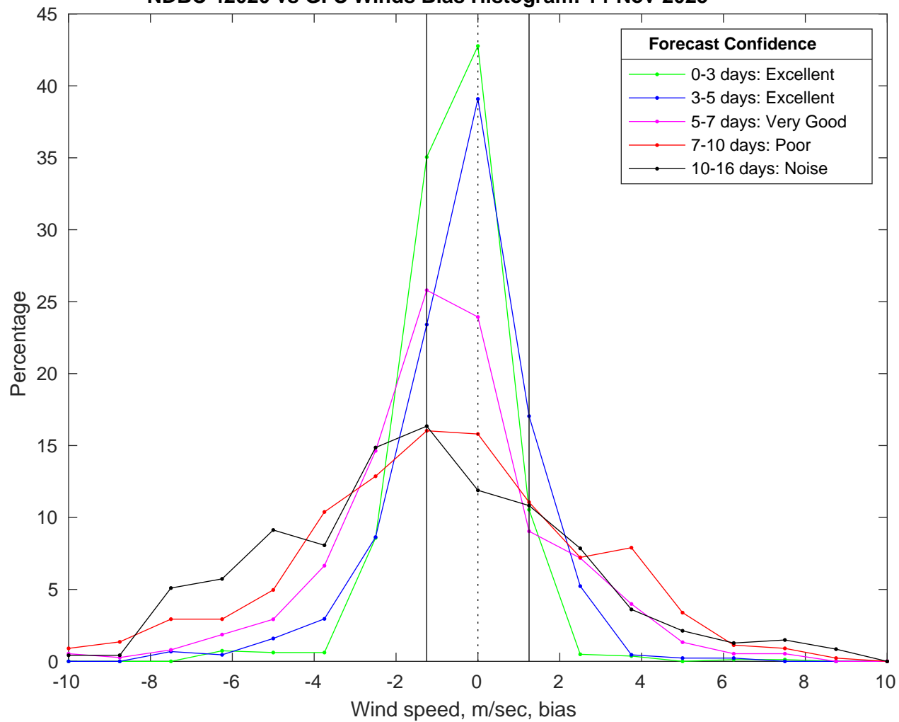
NDBC 42020 vs GFS Winds Bias Histogram: 14-Nov-2025
