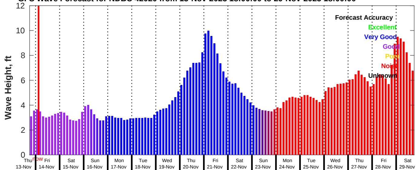
GFS Wave Forecast for NDBC 42020 from 13-Nov-2025 18:00:00 to 29-Nov-2025 18:00:00
