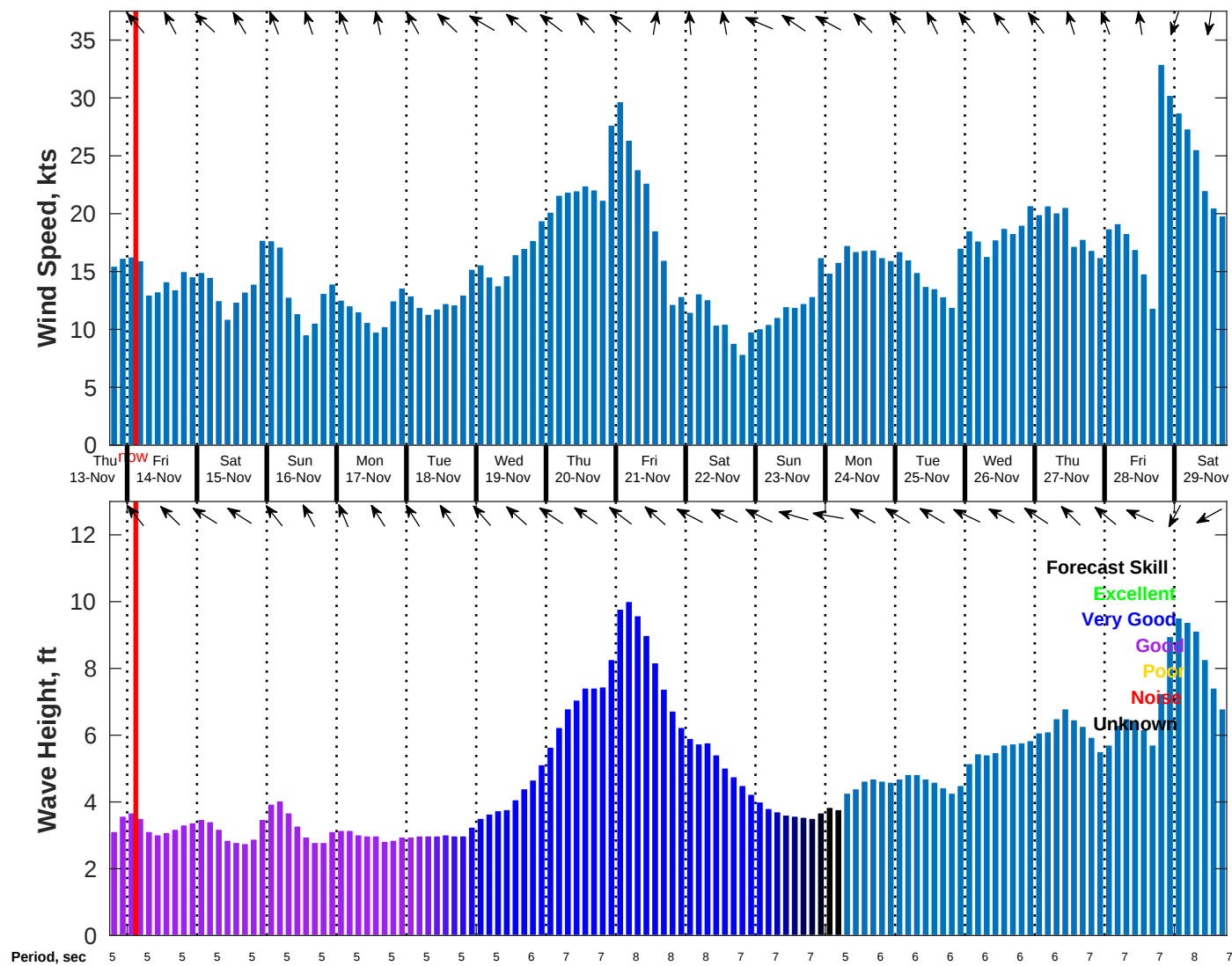
Wind & Wave Forecast for NDBC 42020 from 13-Nov-2025 18:00:00 to 29-Nov-2025 18:00:00
