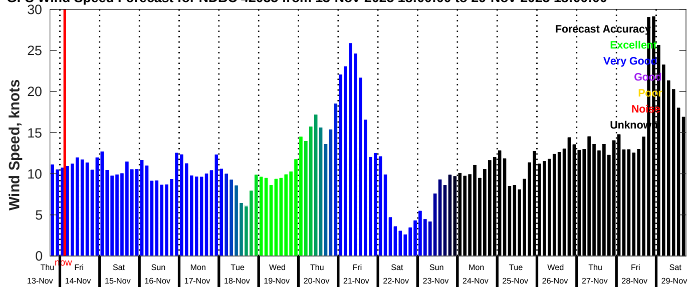
GFS Wind Speed Forecast for NDBC 42035 from 13-Nov-2025 18:00:00 to 29-Nov-2025 18:00:00
