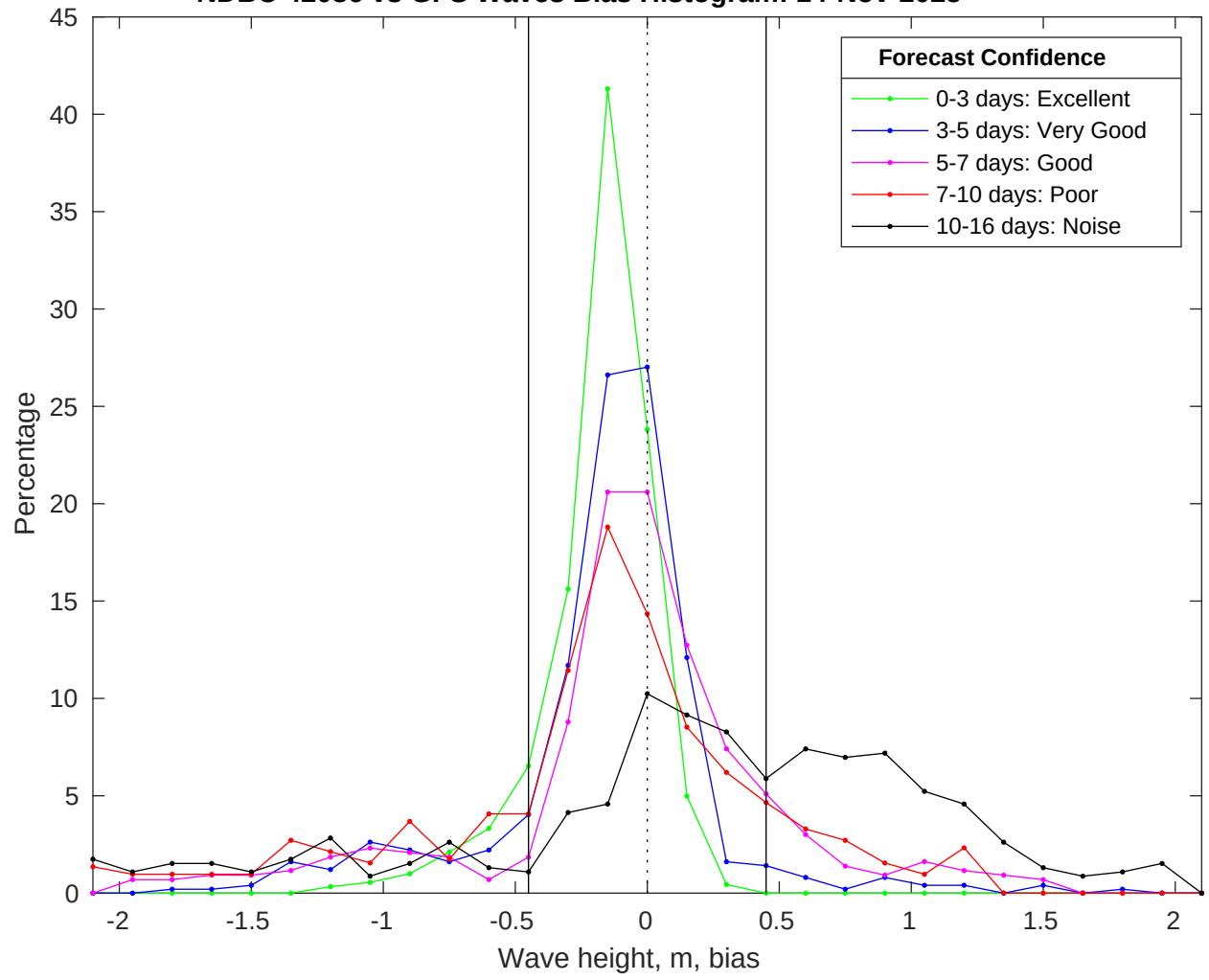
NDBC 42036 vs GFS Waves Bias Histogram: 14-Nov-2025
