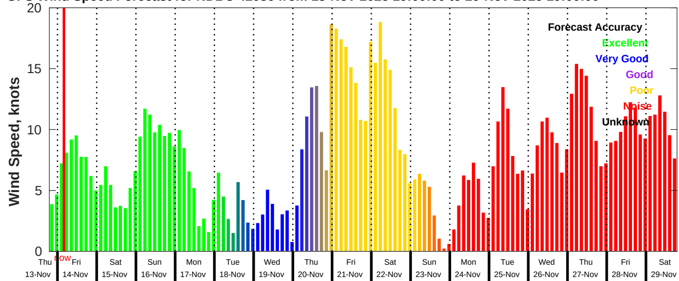
GFS Wind Speed Forecast for NDBC 42036 from 13-Nov-2025 19:00:00 to 29-Nov-2025 19:00:00
