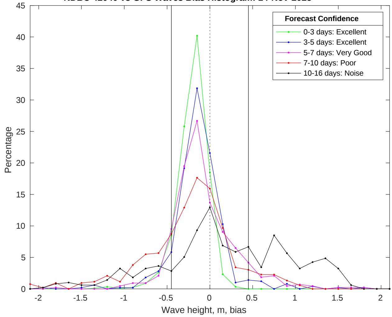
NDBC 42040 vs GFS Waves Bias Histogram: 14-Nov-2025
