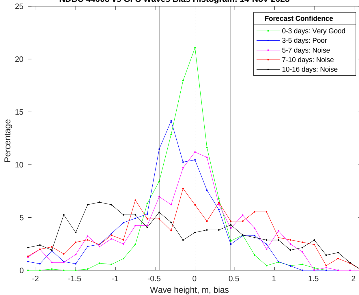
NDBC 44008 vs GFS Waves Bias Histogram: 14-Nov-2025
