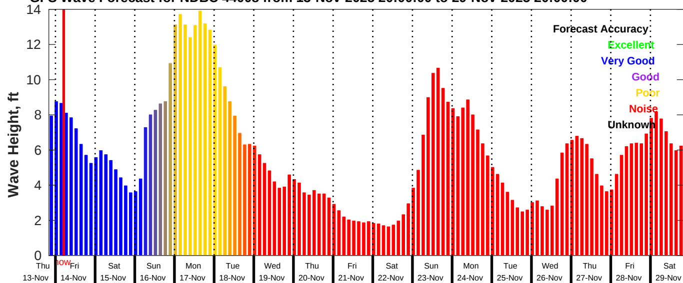
GFS Wave Forecast for NDBC 44008 from 13-Nov-2025 20:00:00 to 29-Nov-2025 20:00:00
