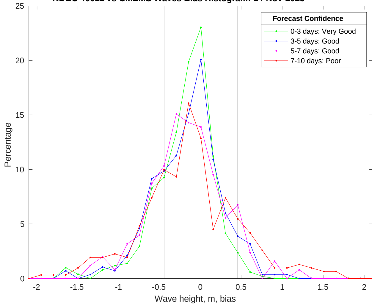
NDBC 46011 vs CMEMS Waves Bias Histogram: 14-Nov-2025
