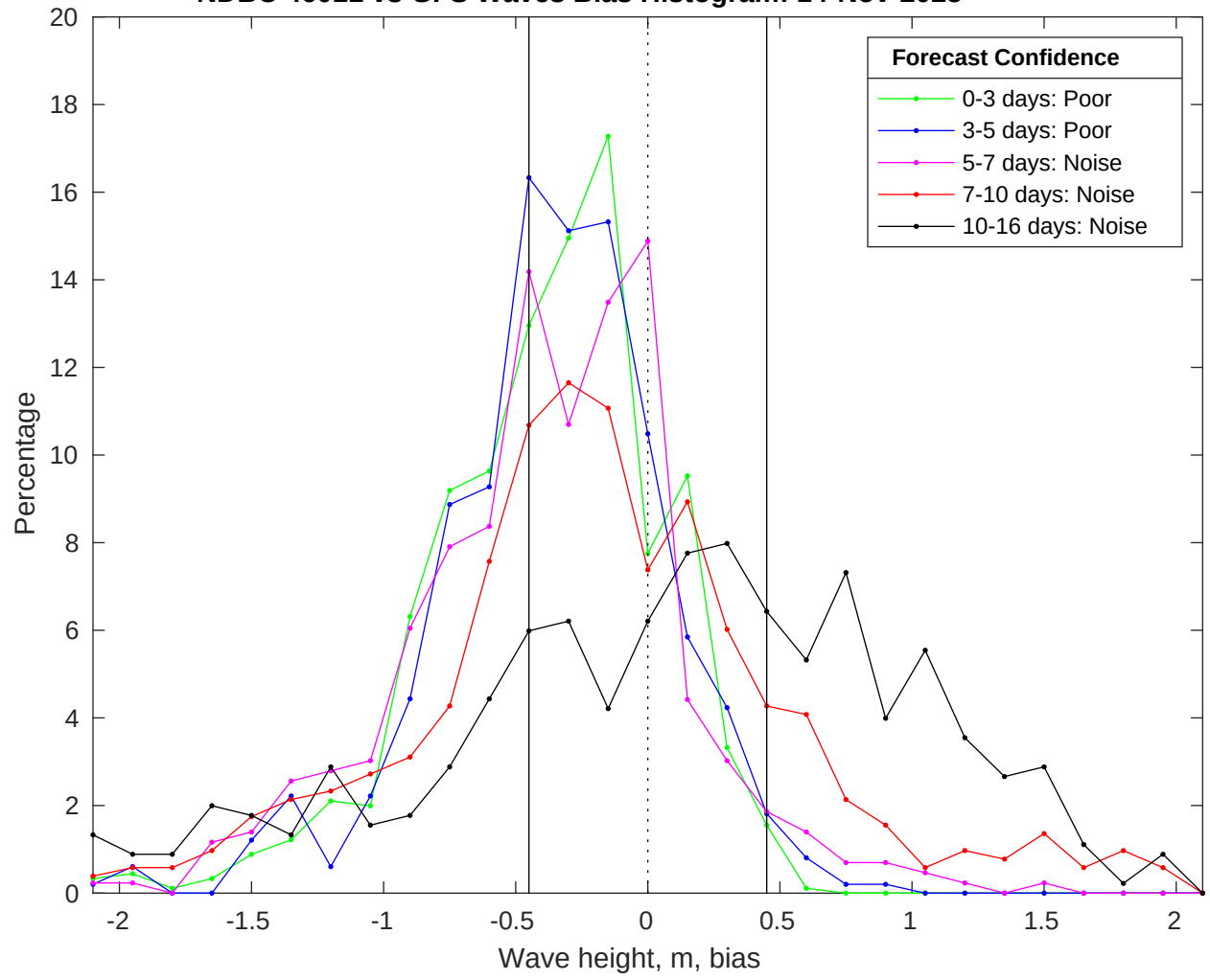
NDBC 46011 vs GFS Waves Bias Histogram: 14-Nov-2025
