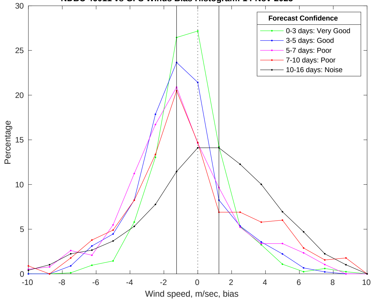
NDBC 46011 vs GFS Winds Bias Histogram: 14-Nov-2025
