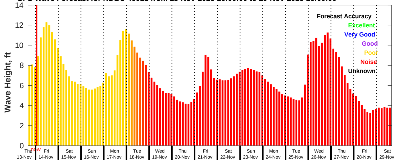
GFS Wave Forecast for NDBC 46011 from 13-Nov-2025 16:00:00 to 29-Nov-2025 16:00:00
