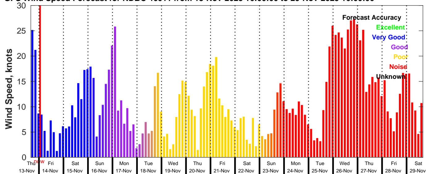
GFS Wind Speed Forecast for NDBC 46011 from 13-Nov-2025 16:00:00 to 29-Nov-2025 16:00:00
