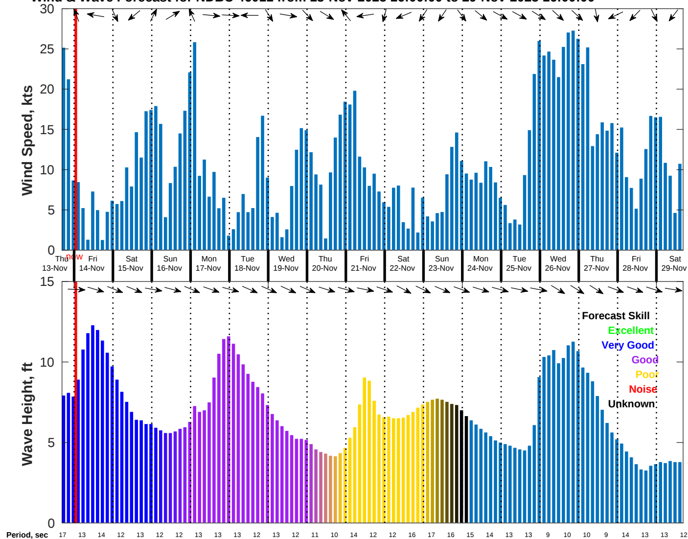
Wind & Wave Forecast for NDBC 46011 from 13-Nov-2025 16:00:00 to 29-Nov-2025 16:00:00
