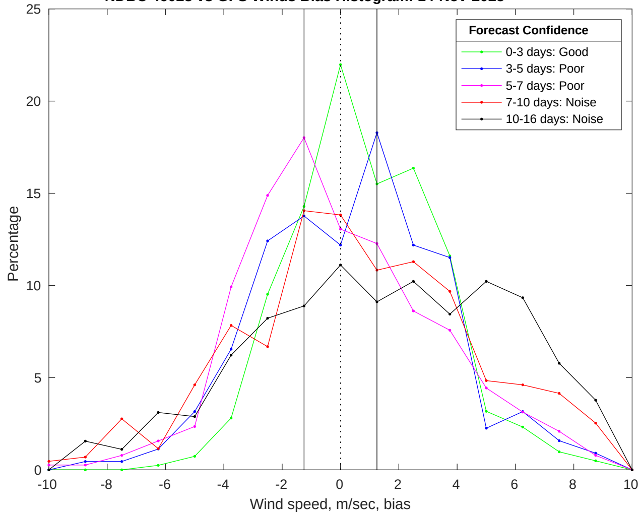
NDBC 46028 vs GFS Winds Bias Histogram: 14-Nov-2025
