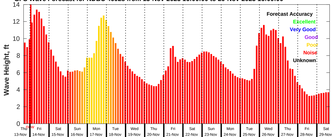
GFS Wave Forecast for NDBC 46028 from 13-Nov-2025 16:00:00 to 29-Nov-2025 16:00:00
