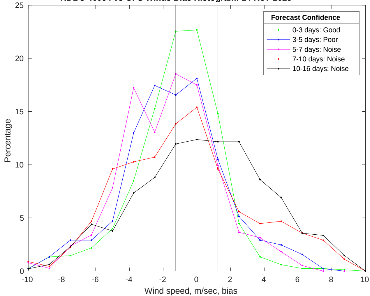
NDBC 46054 vs GFS Winds Bias Histogram: 14-Nov-2025
