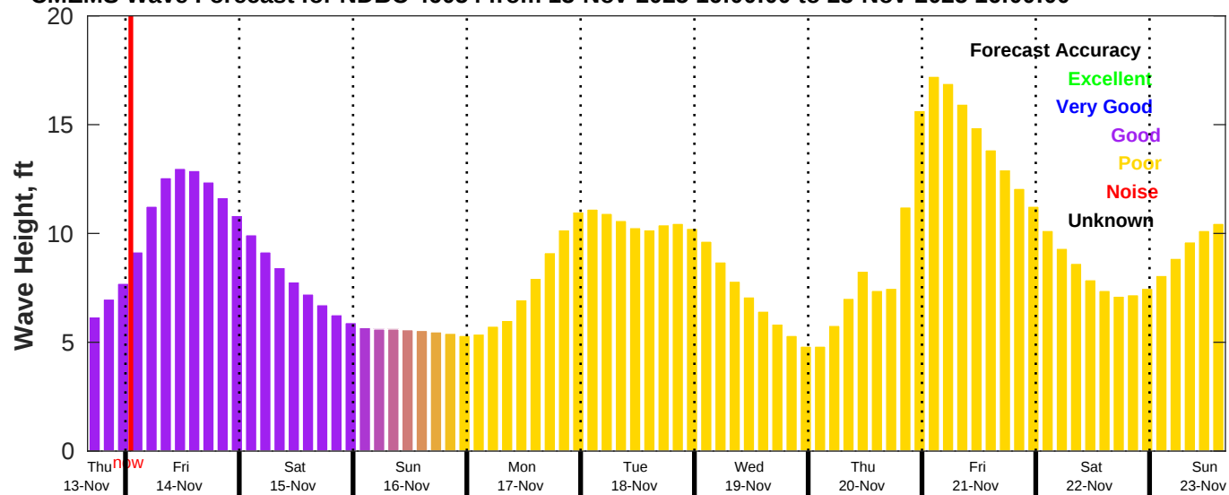
CMEMS Wave Forecast for NDBC 46054 from 13-Nov-2025 16:00:00 to 23-Nov-2025 16:00:00
