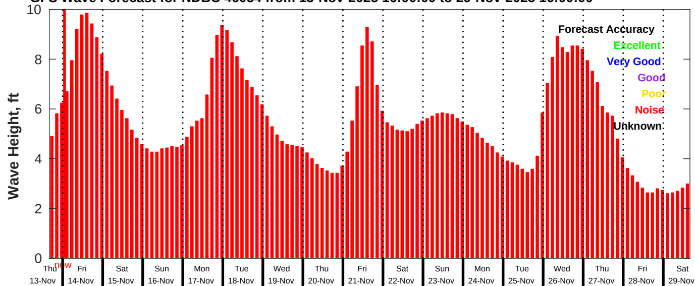
GFS Wave Forecast for NDBC 46054 from 13-Nov-2025 16:00:00 to 29-Nov-2025 16:00:00
