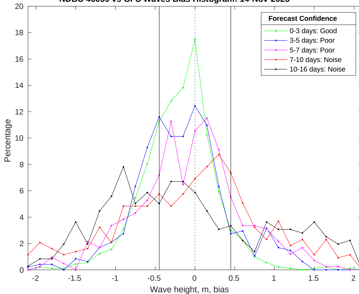
NDBC 46059 vs GFS Waves Bias Histogram: 14-Nov-2025
