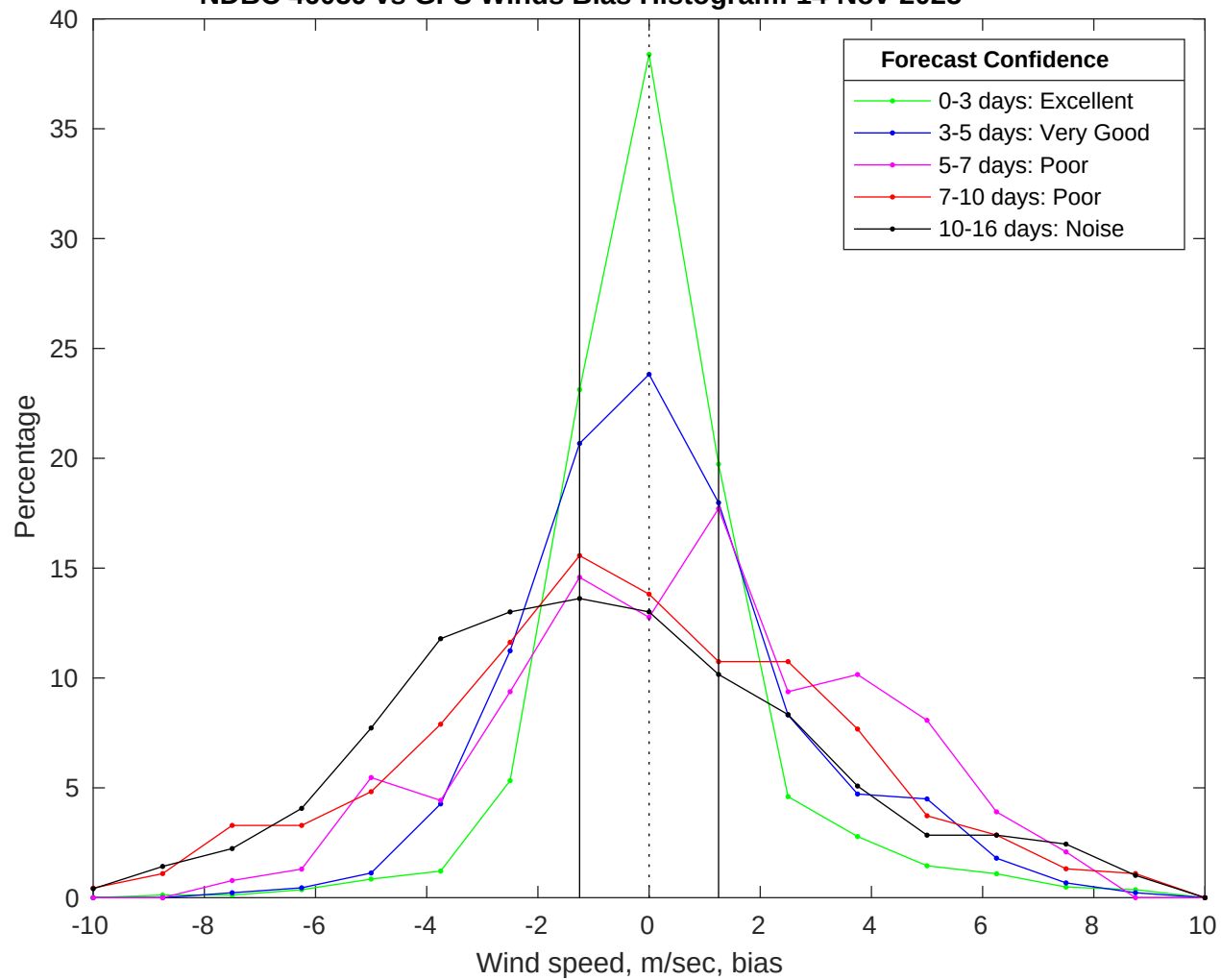
NDBC 46059 vs GFS Winds Bias Histogram: 14-Nov-2025
