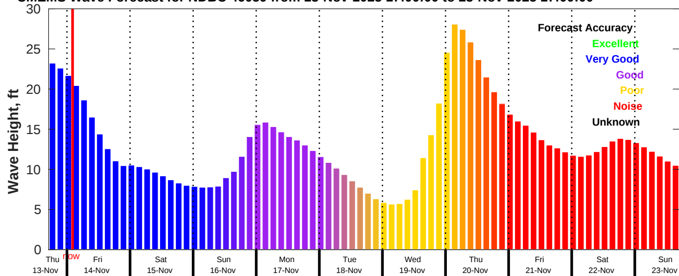
CMEMS Wave Forecast for NDBC 46059 from 13-Nov-2025 17:00:00 to 23-Nov-2025 17:00:00
