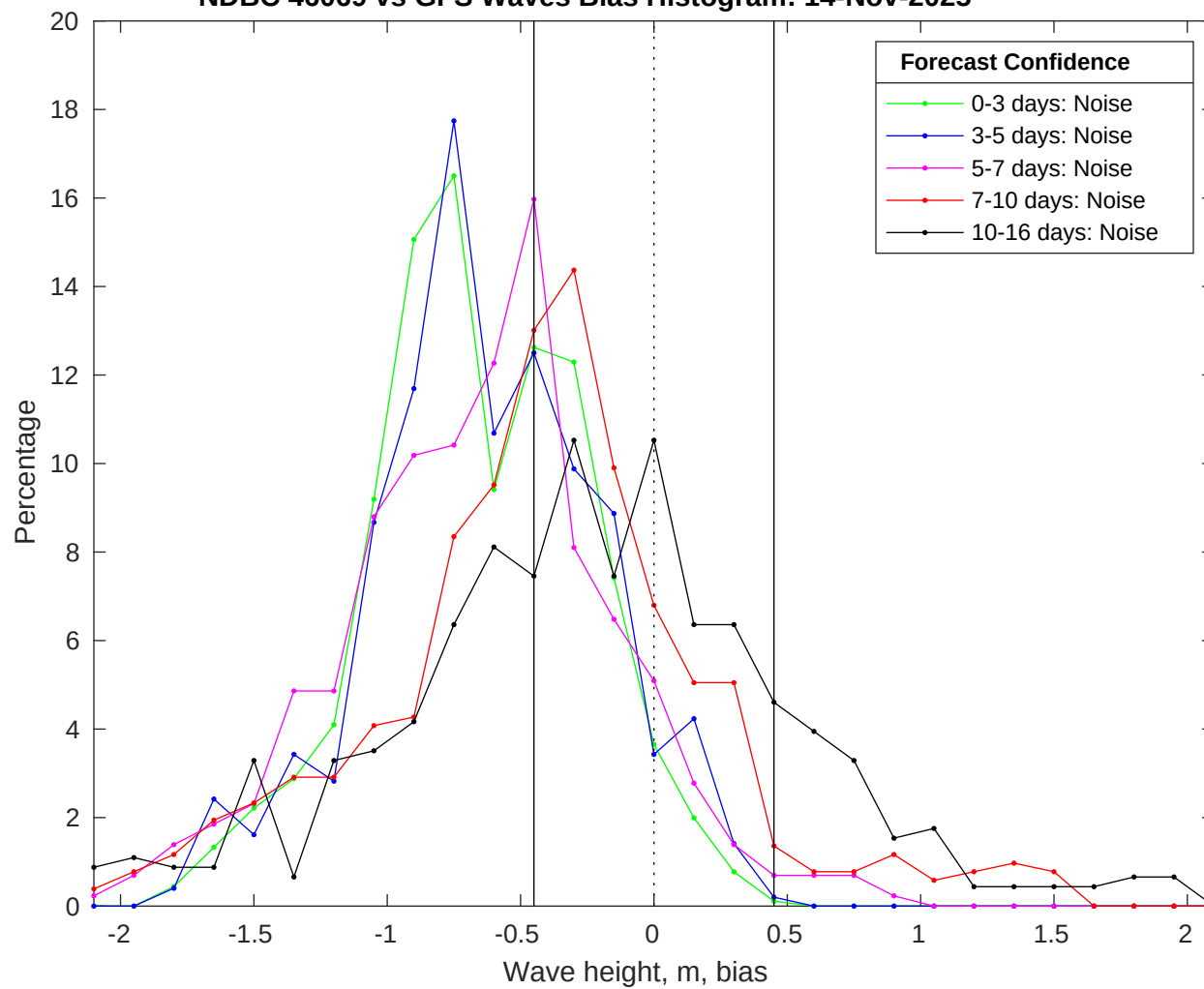
NDBC 46069 vs GFS Waves Bias Histogram: 14-Nov-2025
