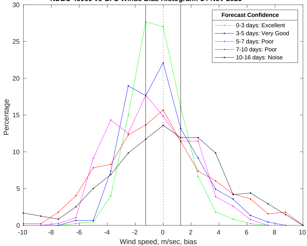
NDBC 46069 vs GFS Winds Bias Histogram: 14-Nov-2025
