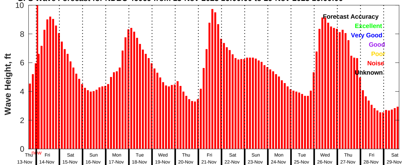
GFS Wave Forecast for NDBC 46069 from 13-Nov-2025 16:00:00 to 29-Nov-2025 16:00:00
