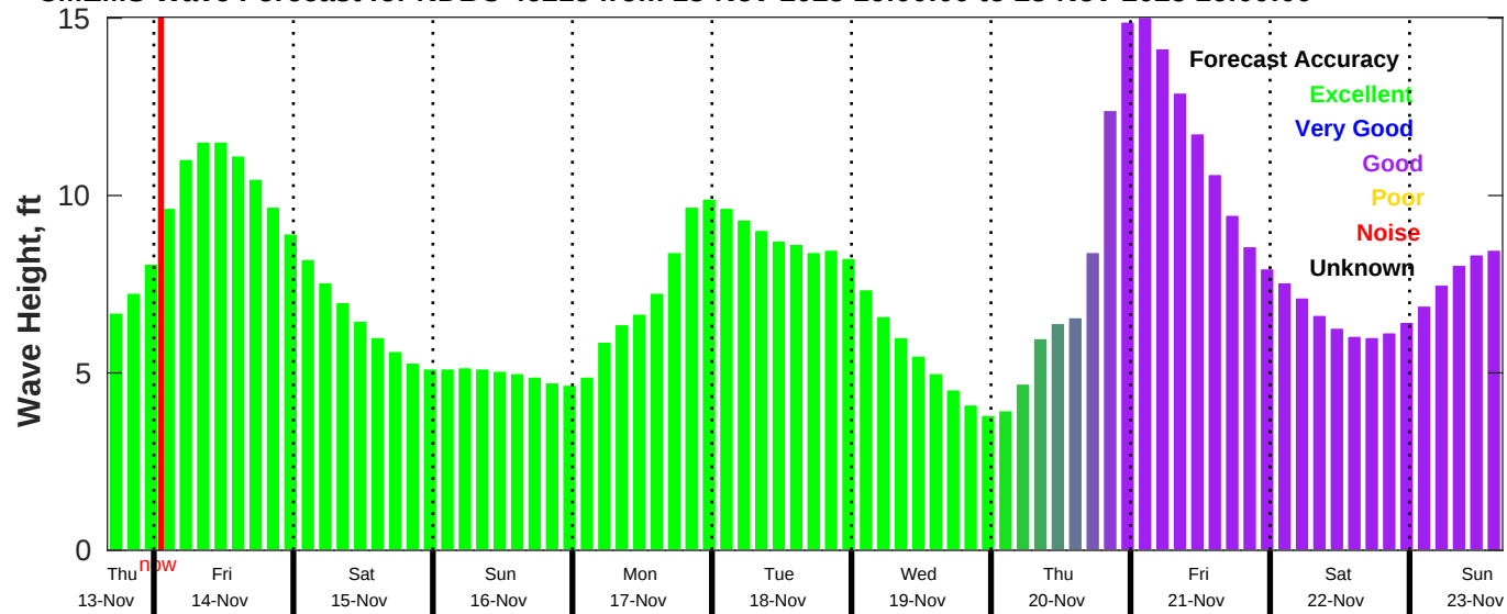
CMEMS Wave Forecast for NDBC 46215 from 13-Nov-2025 16:00:00 to 23-Nov-2025 16:00:00
