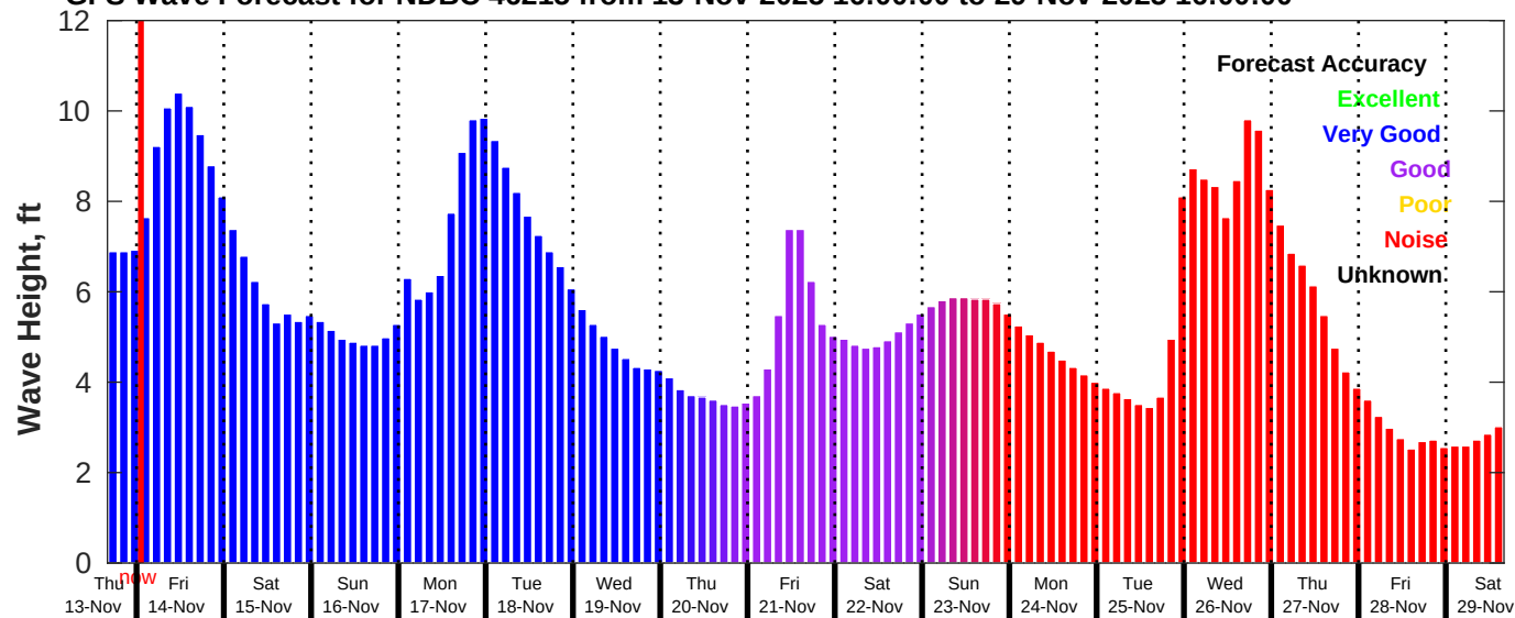
GFS Wave Forecast for NDBC 46215 from 13-Nov-2025 16:00:00 to 29-Nov-2025 16:00:00
