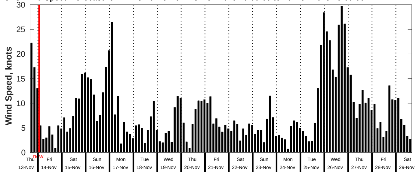
GFS Wind Speed Forecast for NDBC 46215 from 13-Nov-2025 16:00:00 to 29-Nov-2025 16:00:00
