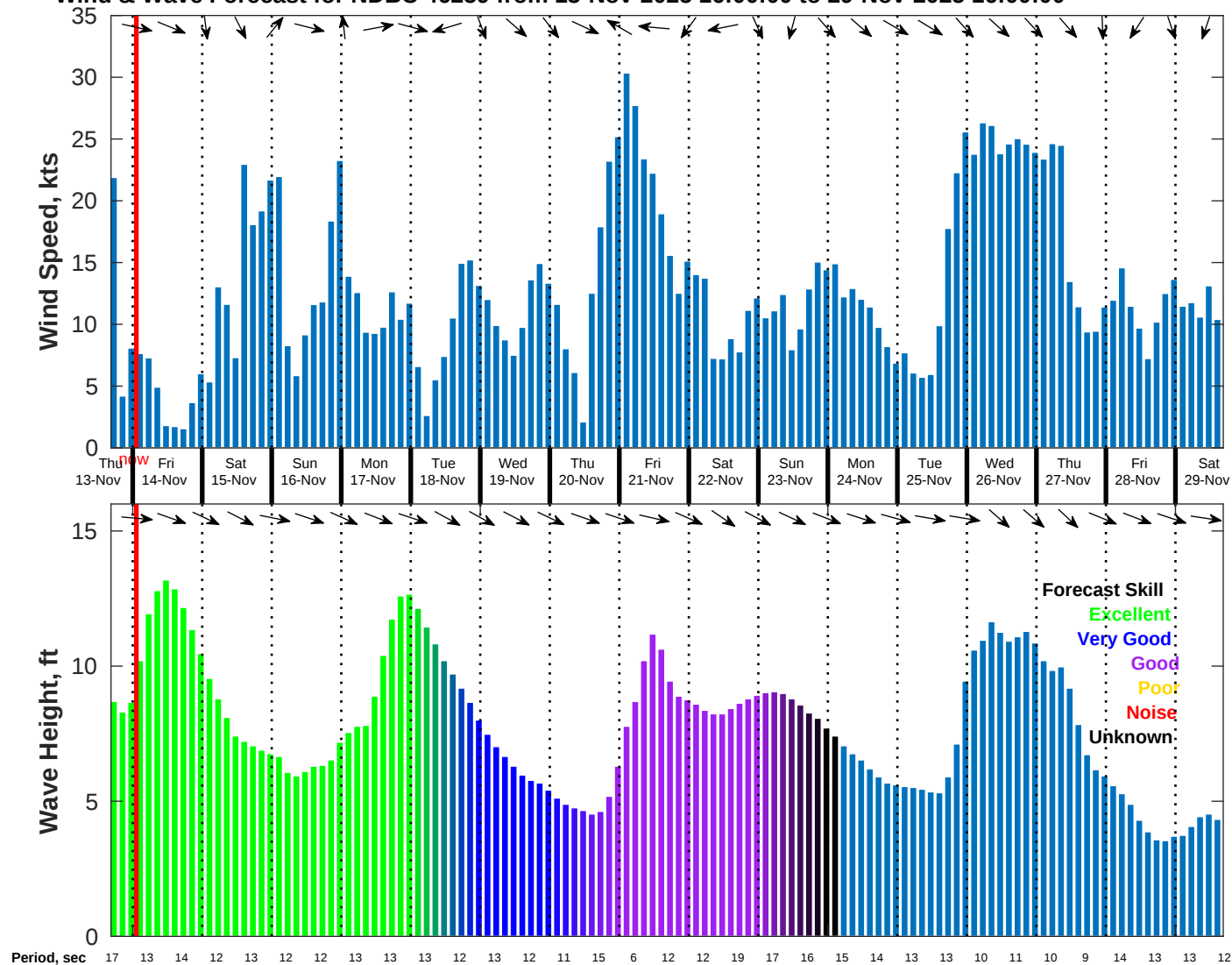
Wind & Wave Forecast for NDBC 46259 from 13-Nov-2025 16:00:00 to 29-Nov-2025 16:00:00
