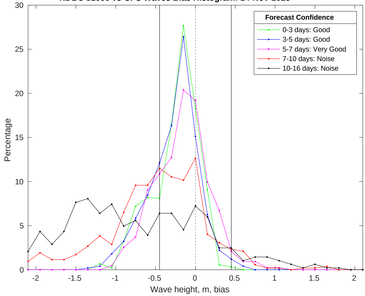
NDBC 51000 vs GFS Waves Bias Histogram: 14-Nov-2025
