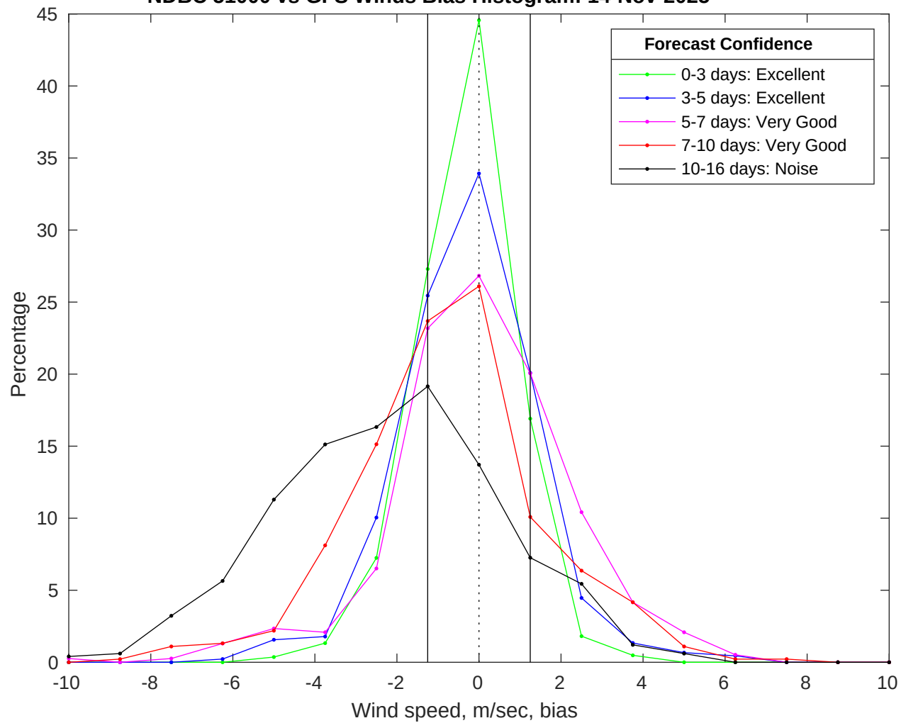
NDBC 51000 vs GFS Winds Bias Histogram: 14-Nov-2025
