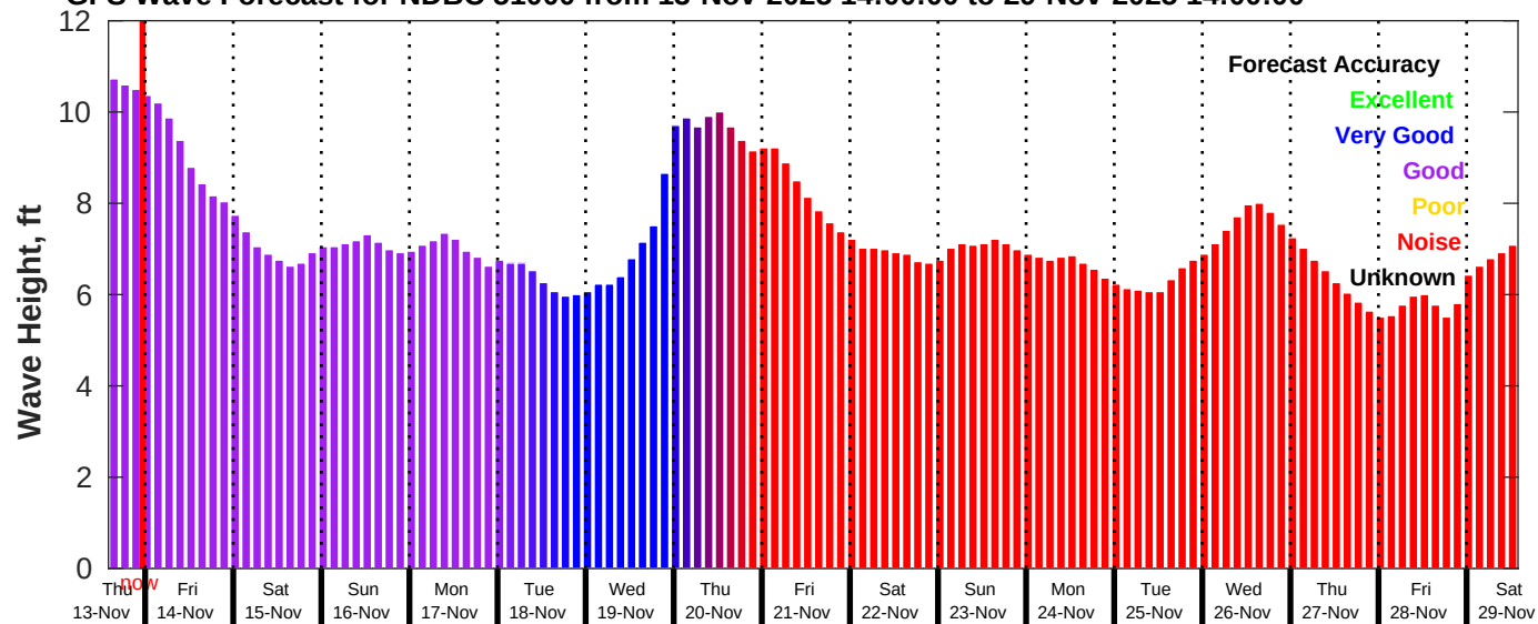
GFS Wave Forecast for NDBC 51000 from 13-Nov-2025 14:00:00 to 29-Nov-2025 14:00:00
