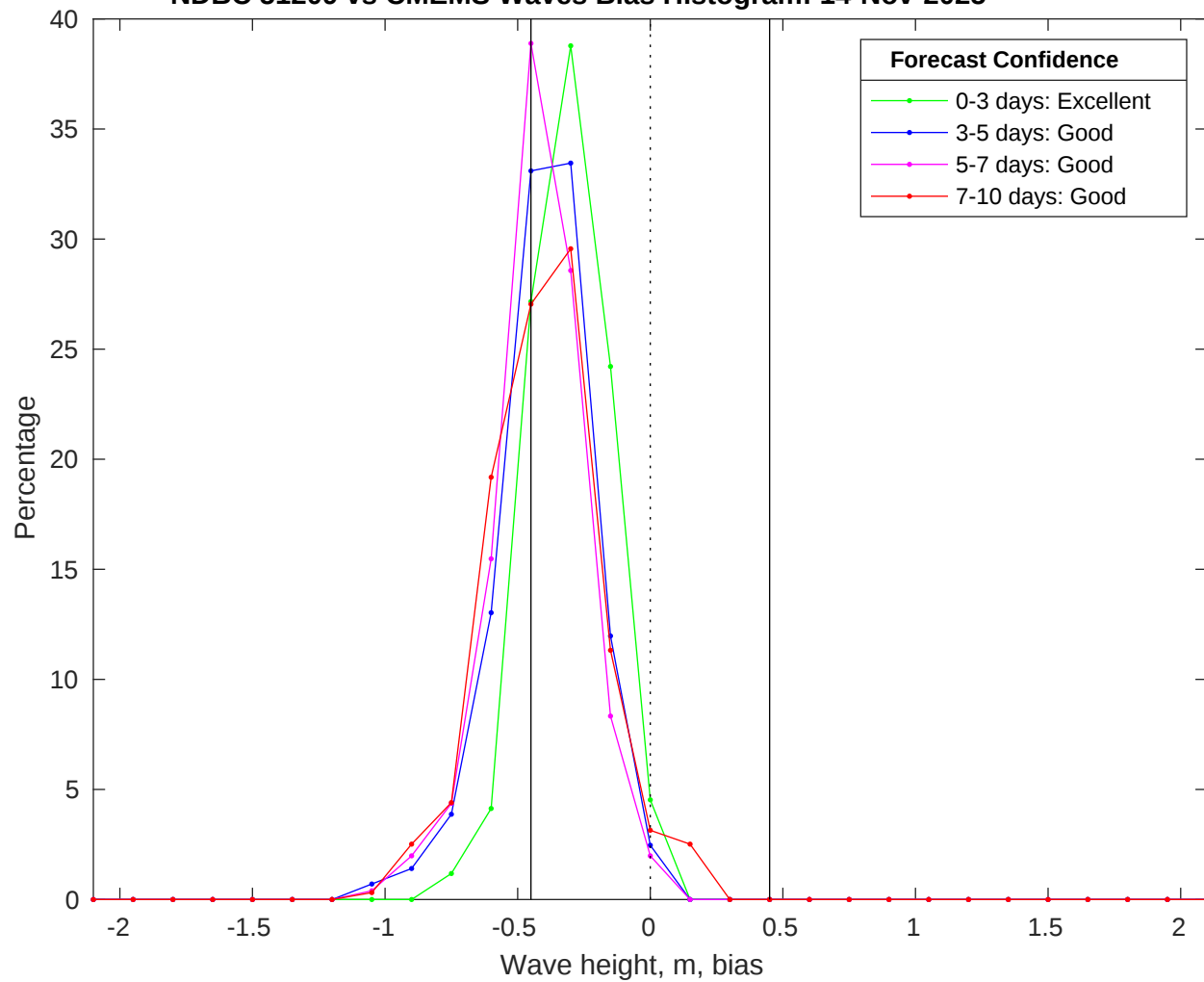
NDBC 51209 vs CMEMS Waves Bias Histogram: 14-Nov-2025
