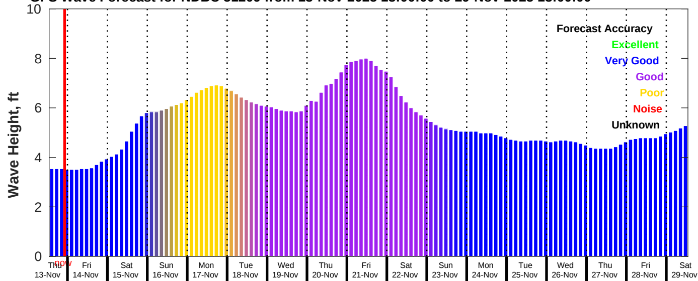
GFS Wave Forecast for NDBC 51209 from 13-Nov-2025 13:00:00 to 29-Nov-2025 13:00:00
