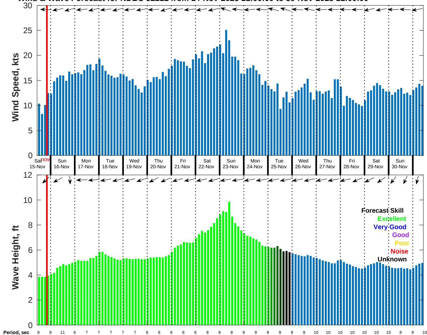
Wind & Wave Forecast for NDBC 52211 from 14-Nov-2025 11:00:00 to 30-Nov-2025 11:00:00
