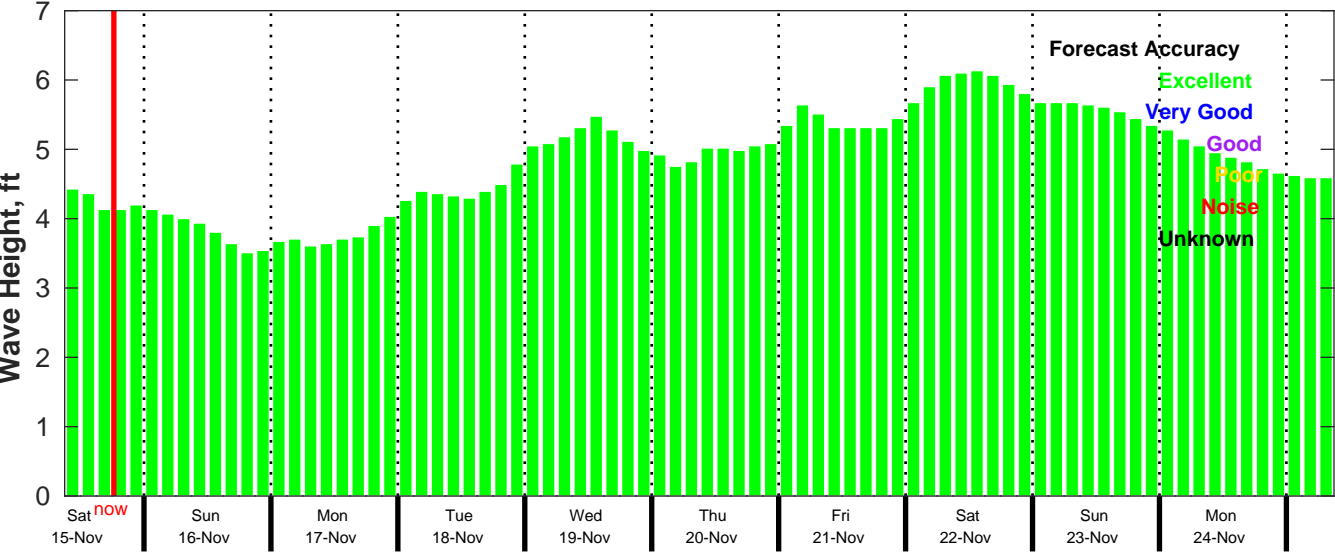
CMEMS Wave Forecast for NDBC 52212 from 14-Nov-2025 09:00:00 to 24-Nov-2025 09:00:00
